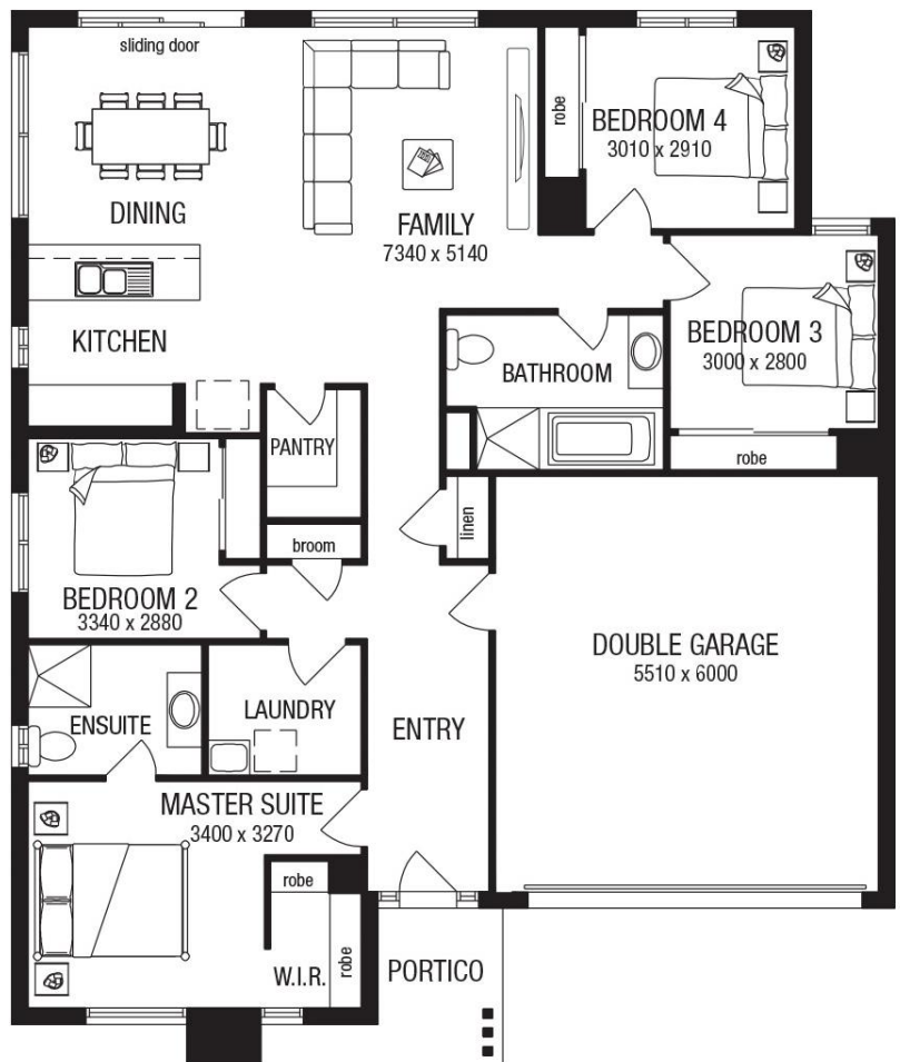
Floor plan and standard specification shown. Floor plan may not reflect developer guidelines
